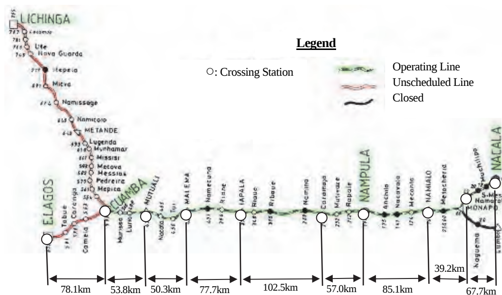
Figure 1.3 Northern Railway in Mozambique
